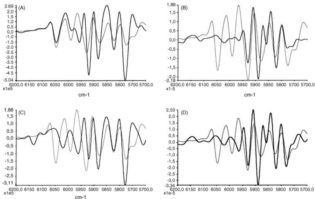
Fig. 6. Second-derivative spectra of a reference Viagra ® tablet (dashed) and of four different sample tablets, sample code 6817 (A); sample code 5471 (B); sample code 6816 (C); and sample code 5472 (D).
